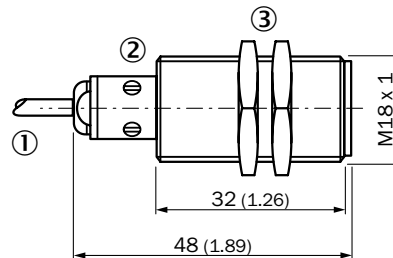
All dimensions in mm (inch)
