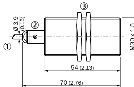
IME30-xxBxxW2S, flush, cable, standard
