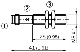
IME08-xBxxxTOK, flush, connector, short-body housing
