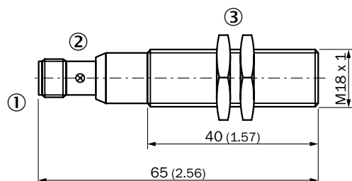
All dimensions in mm (inch)
