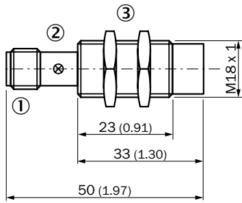
All dimensions in mm (inch)
