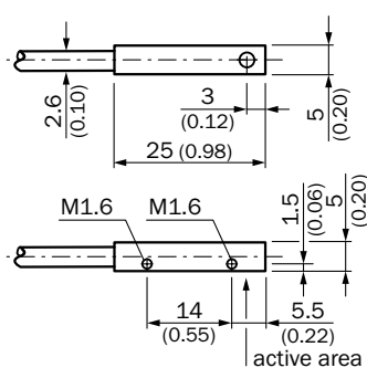
IQ05-xx8xx-ZU1, flush, cable
