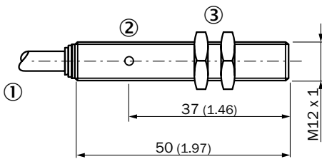
All dimensions in mm (inch)
