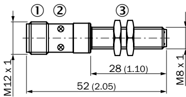
IME08-xBxxxC0S, flush, connector M12, standard
