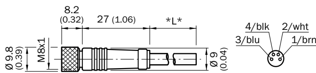
All dimensions in mm (inch)
