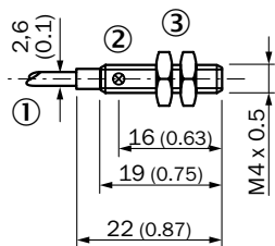
IM04, cable
