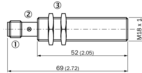
IME18-xxBxxxC0S, flush, connector, standard
