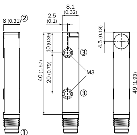
IQ08-xxxxxxT0S, connector
