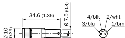
Dimensions in mm (inch)
