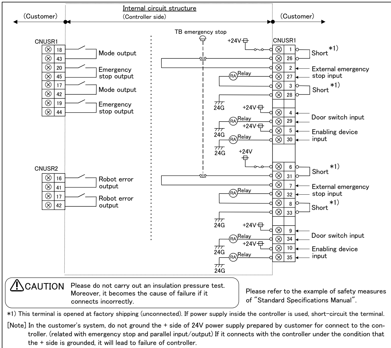
Appendix Fig. 7-15: External emergency stop connection (CR751 controller)
